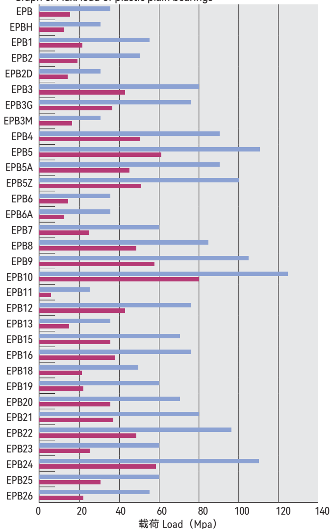
Graph 6: Max. load of plastic plain bearings
