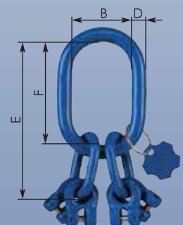
Fixed Size Master Link Assembly TWN 1810/4
