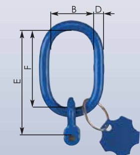
Fixed Size Master Link Assembly TWN 1810/1
