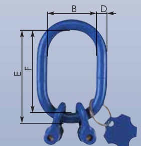
Fixed Size Master Link Assembly TWN 1810/2
