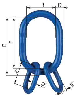
Master Link Assembly TWN 1809
