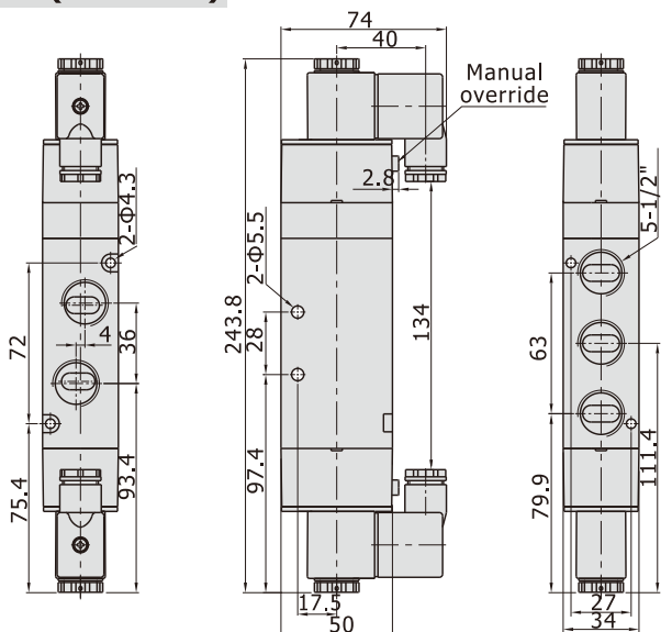
4V430(Terminal)
