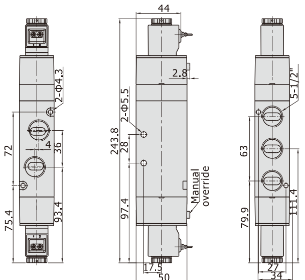
4V430(Flying leads)
