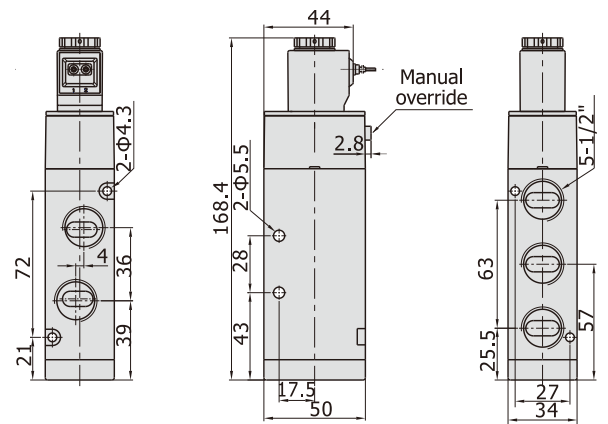
4V420(Flying leads)
