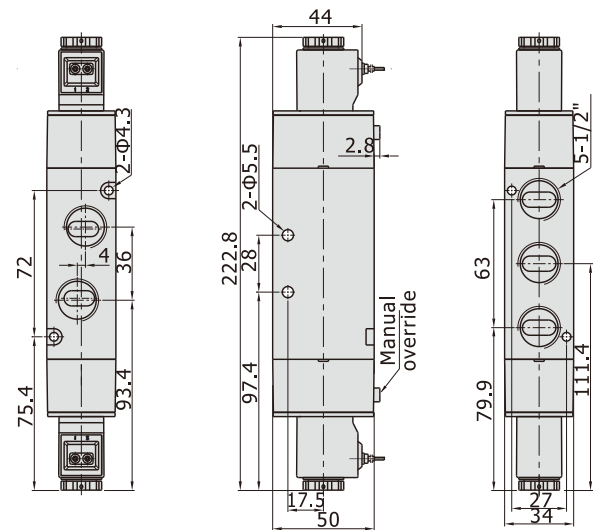
4V430(Flying leads)
