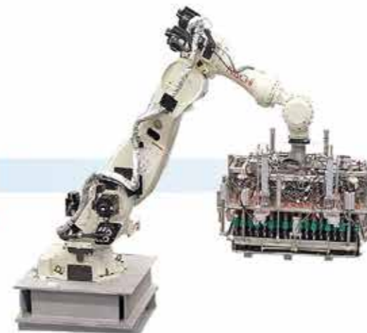
PALLETIZING & DEPALLETIZING FOR USED GLASS BOTTLES (BEER BOTTLES)
