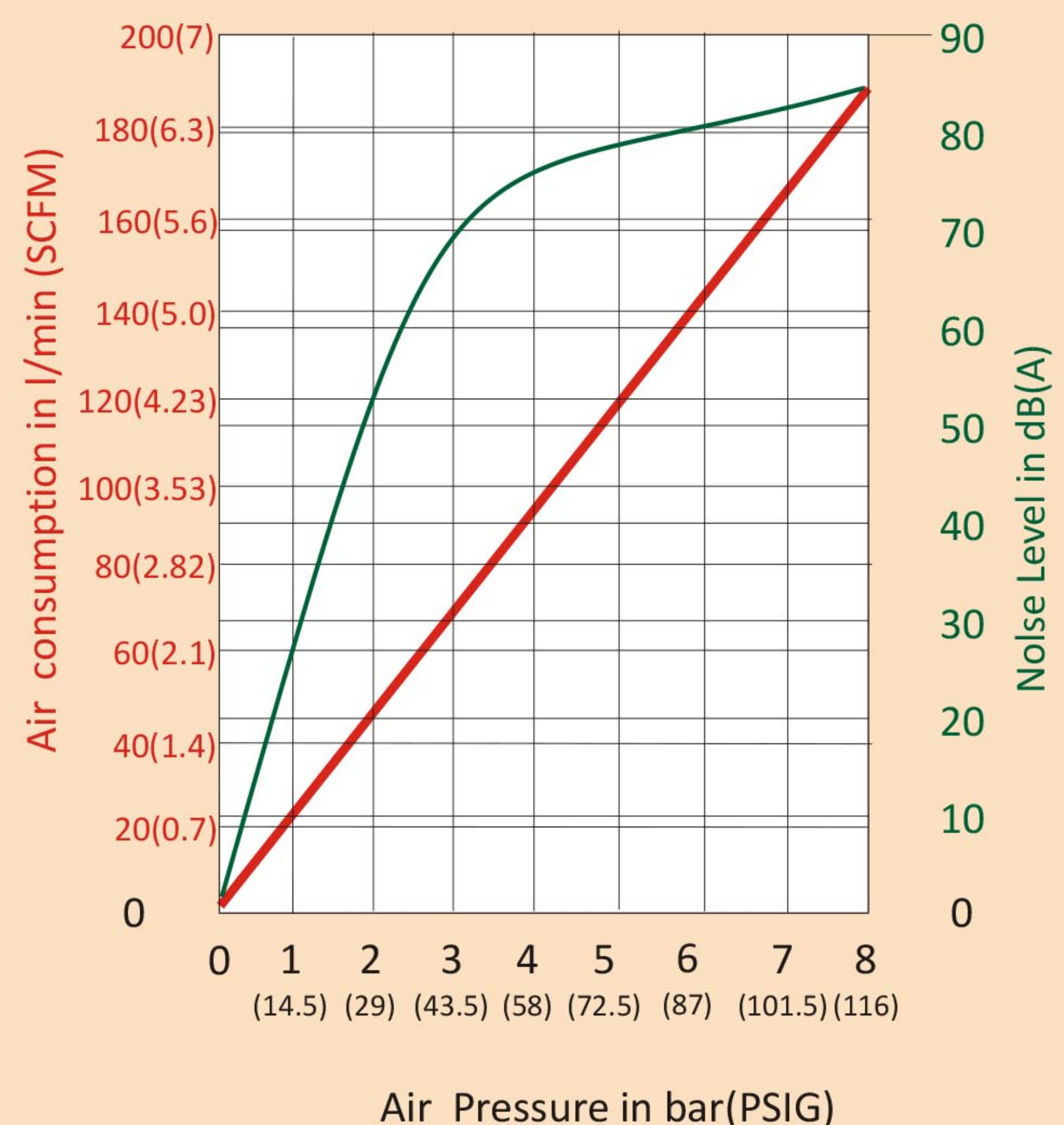
RI LG : Air consumption and noise level
