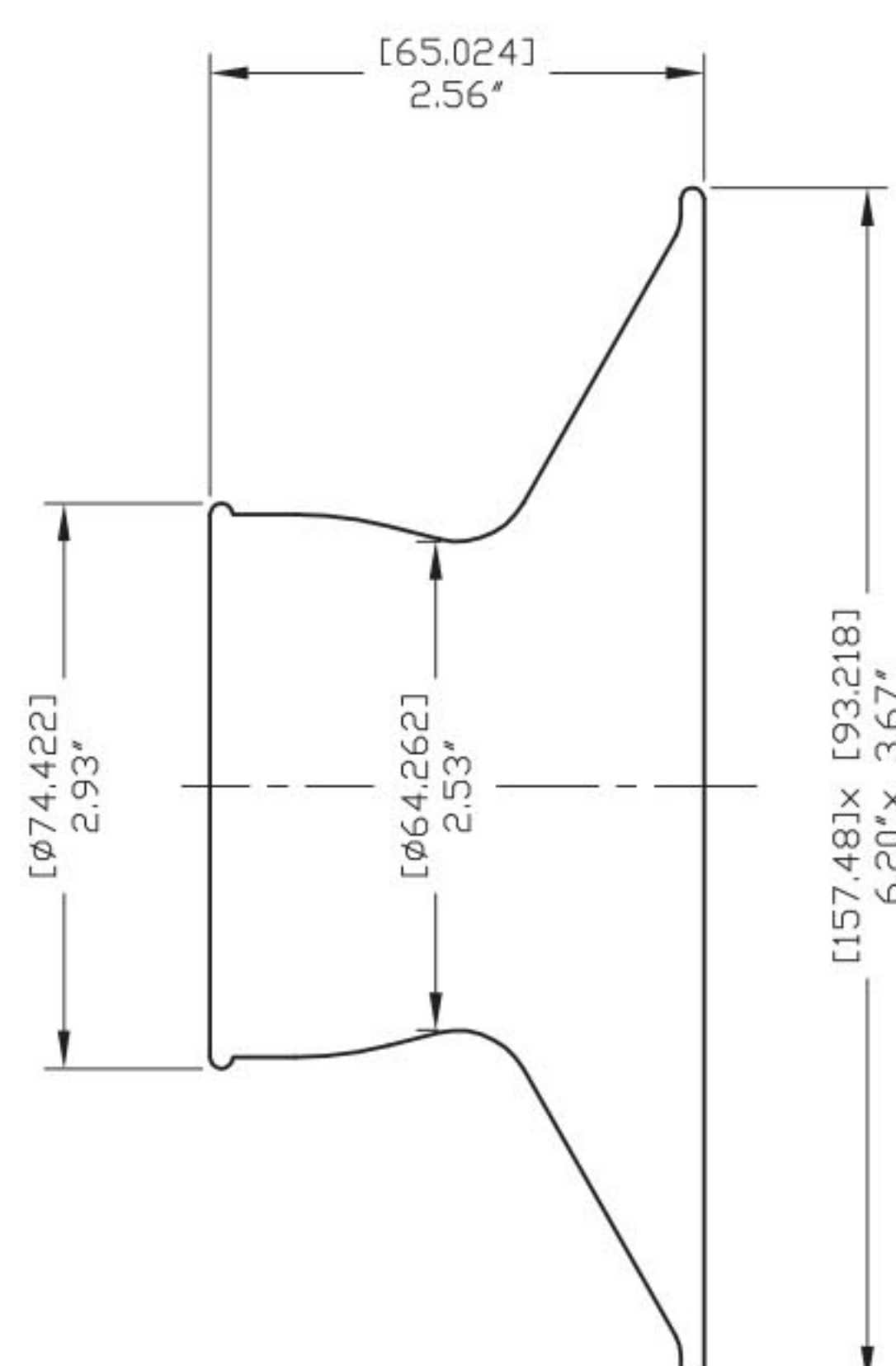
58883 - RECTANGULAR NOZZLE
