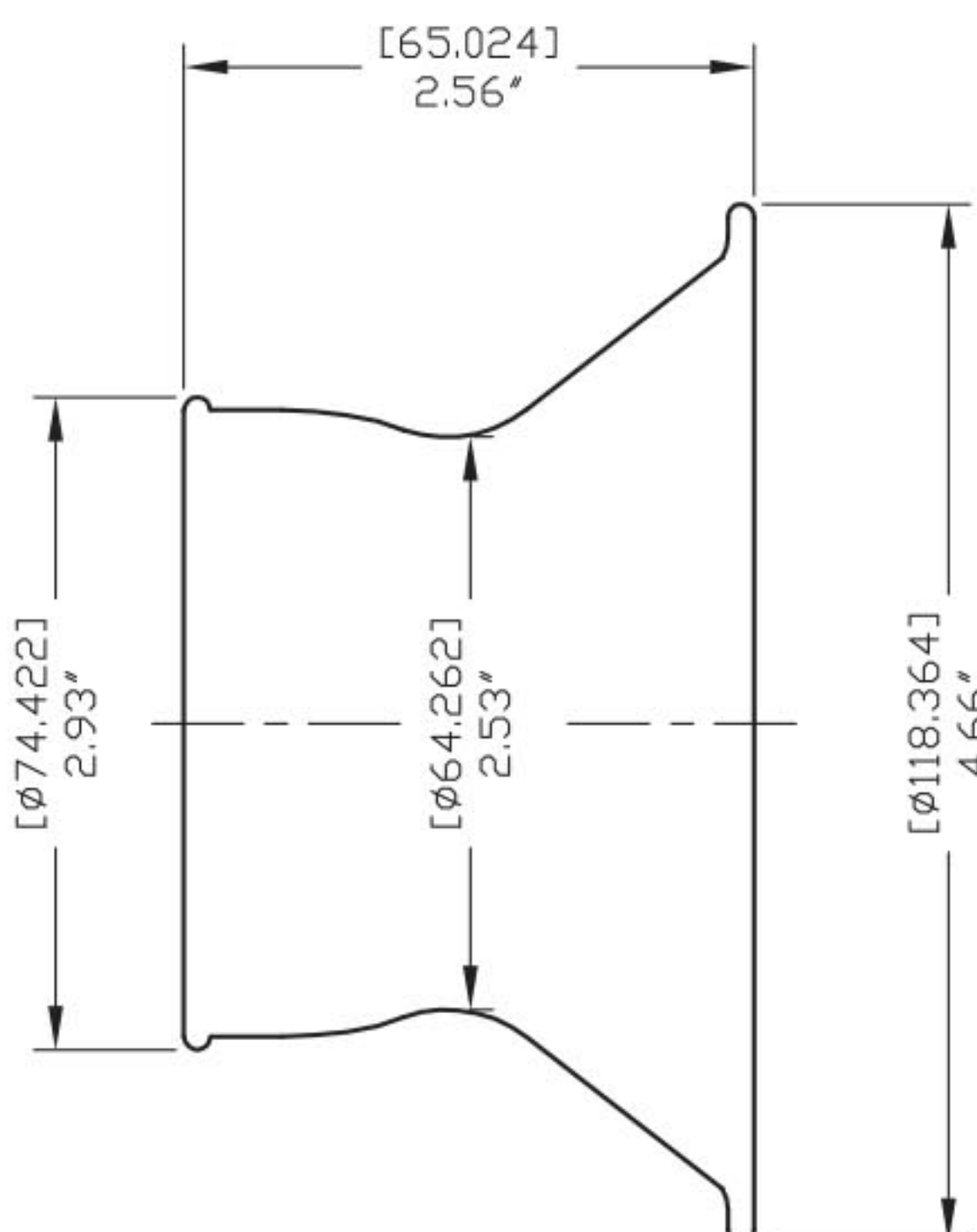
58882 - ROUND NOZZLE
