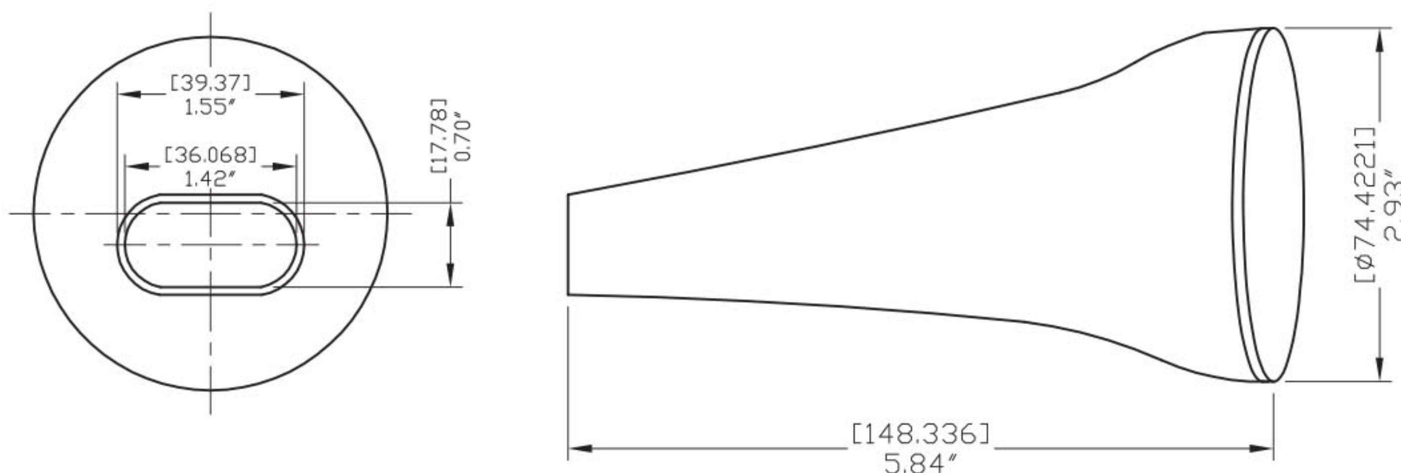
58884 - TAPERED NOZZLE
