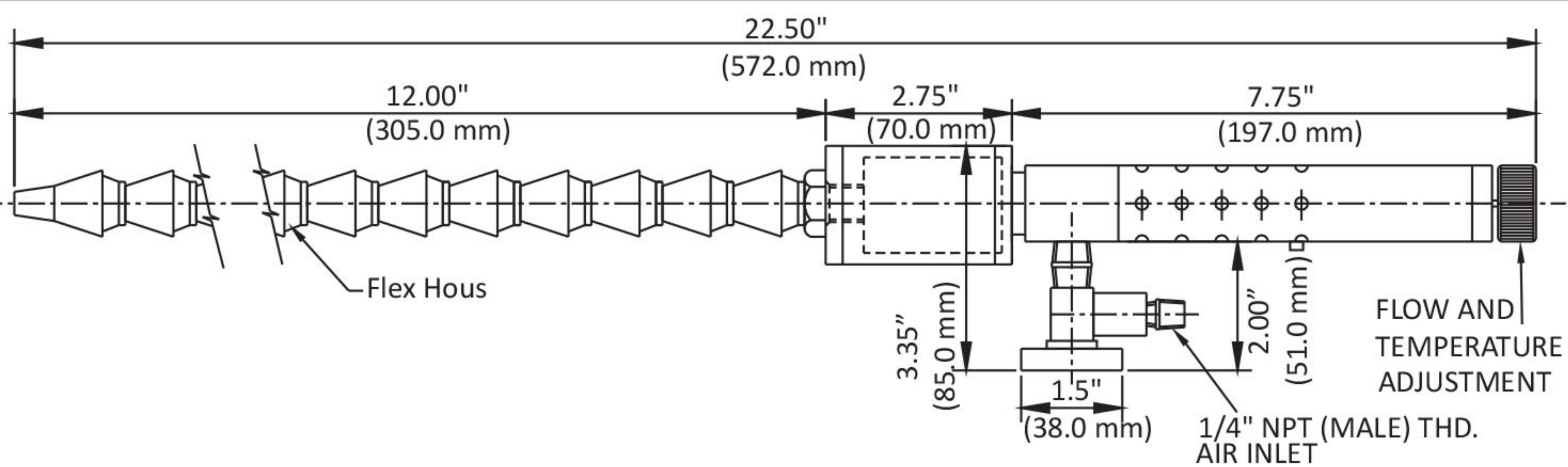
FRIGID-X ADUSTABLE SPOT COOLER
