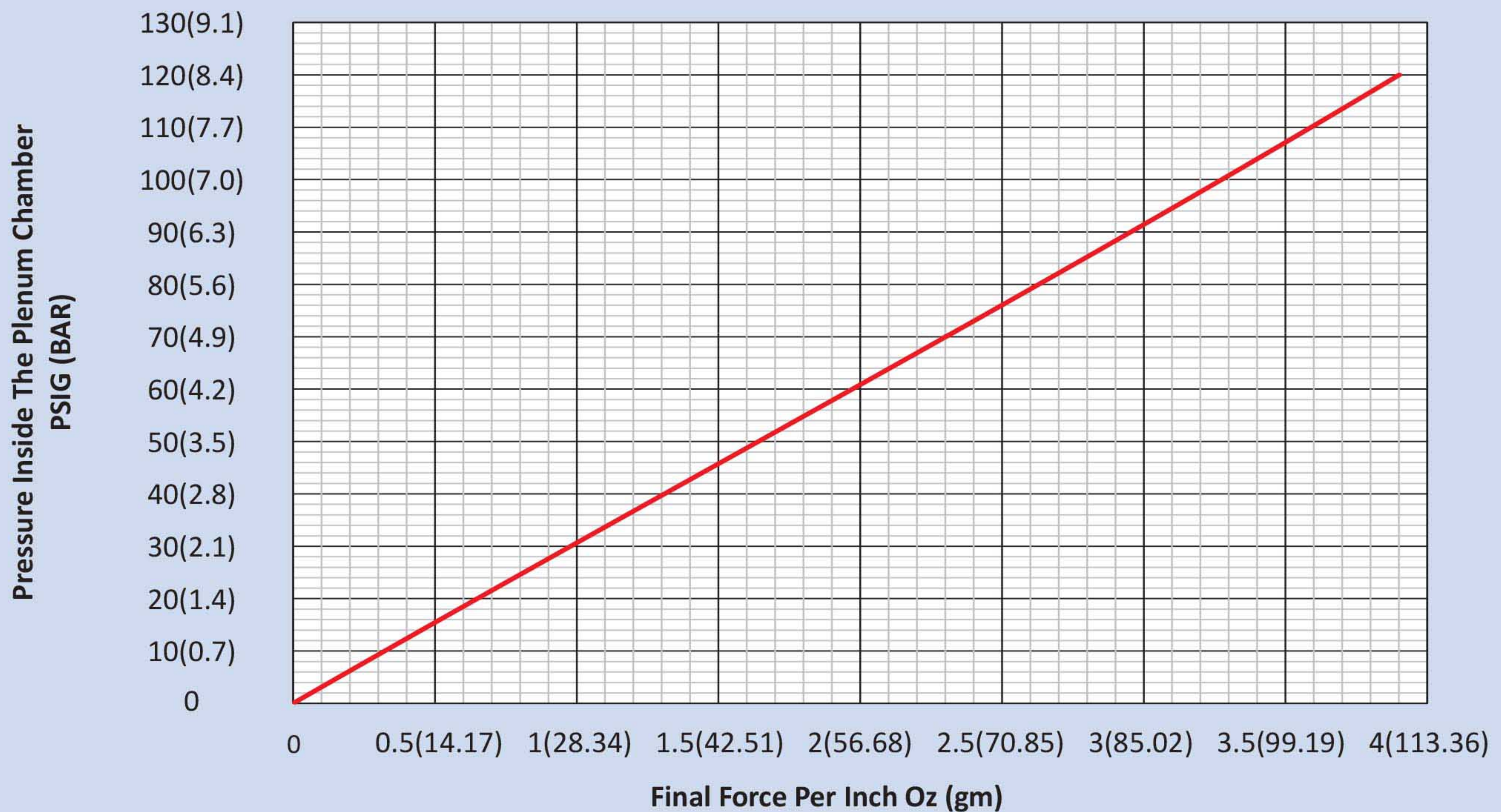
Actual Force Per Inch for Standard Air Blade™ Air Knife
