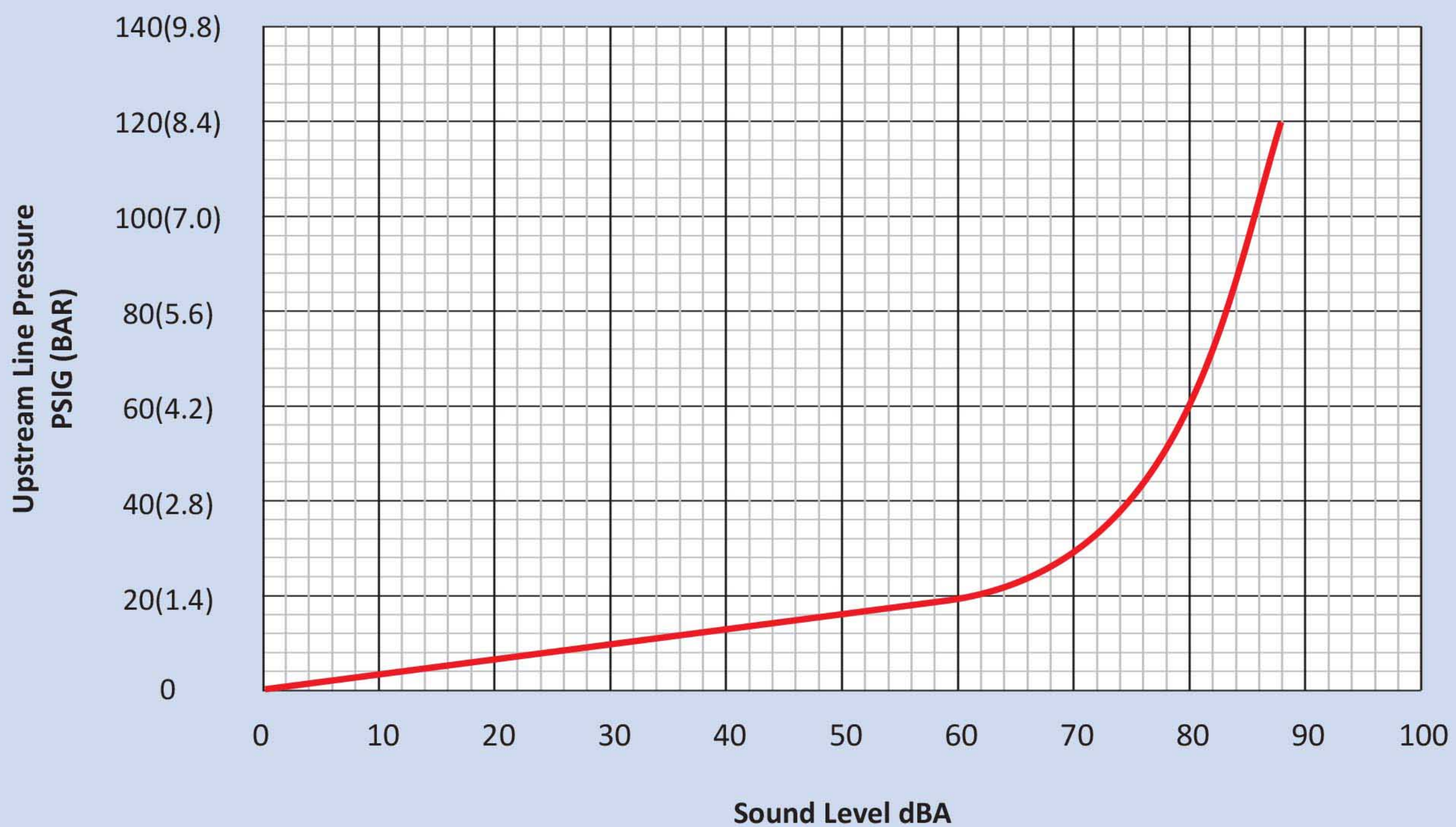
Inlet Pressure Upstream vs. Sound level at 3 feet (0.91m) For Standard Air Blade™ Air Knife
