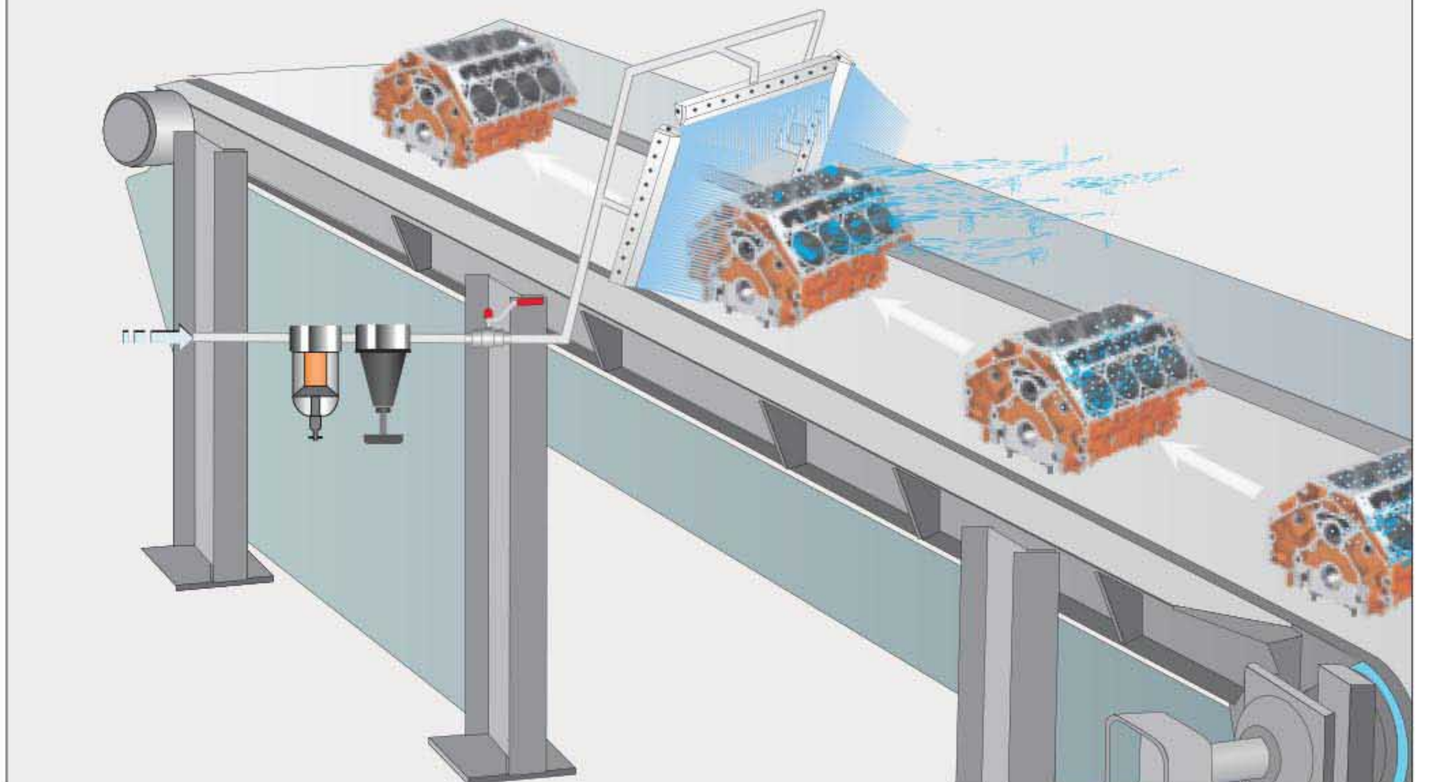
Coolant is blown off of an engine block using three Model 10012X - 12" Silent X-Stream™ Air Blade™ Air Knives
