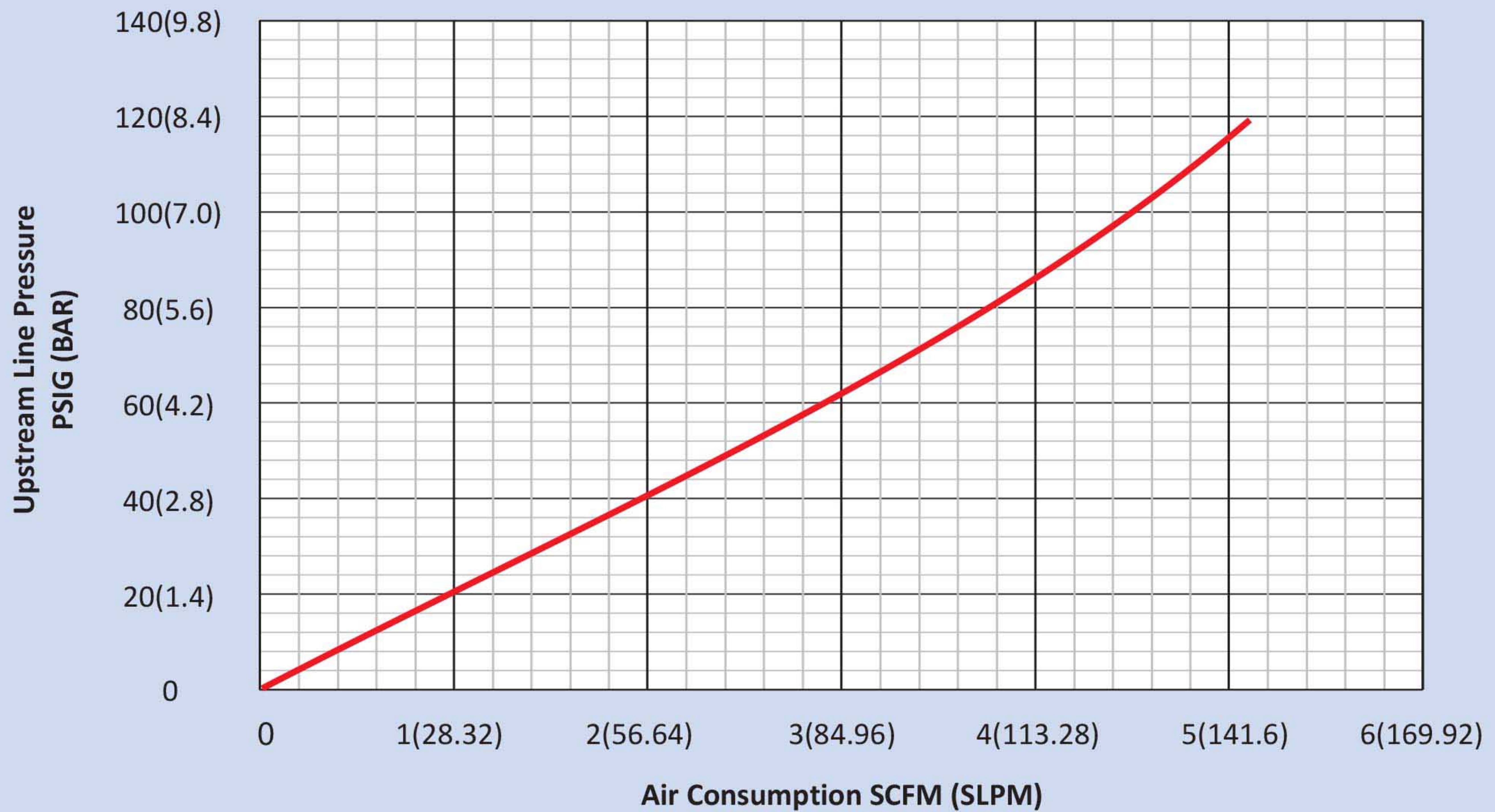
Inlet Pressure Upstream vs. Air Consumption Per Inch for Standard Air Blade™ Air Knife
