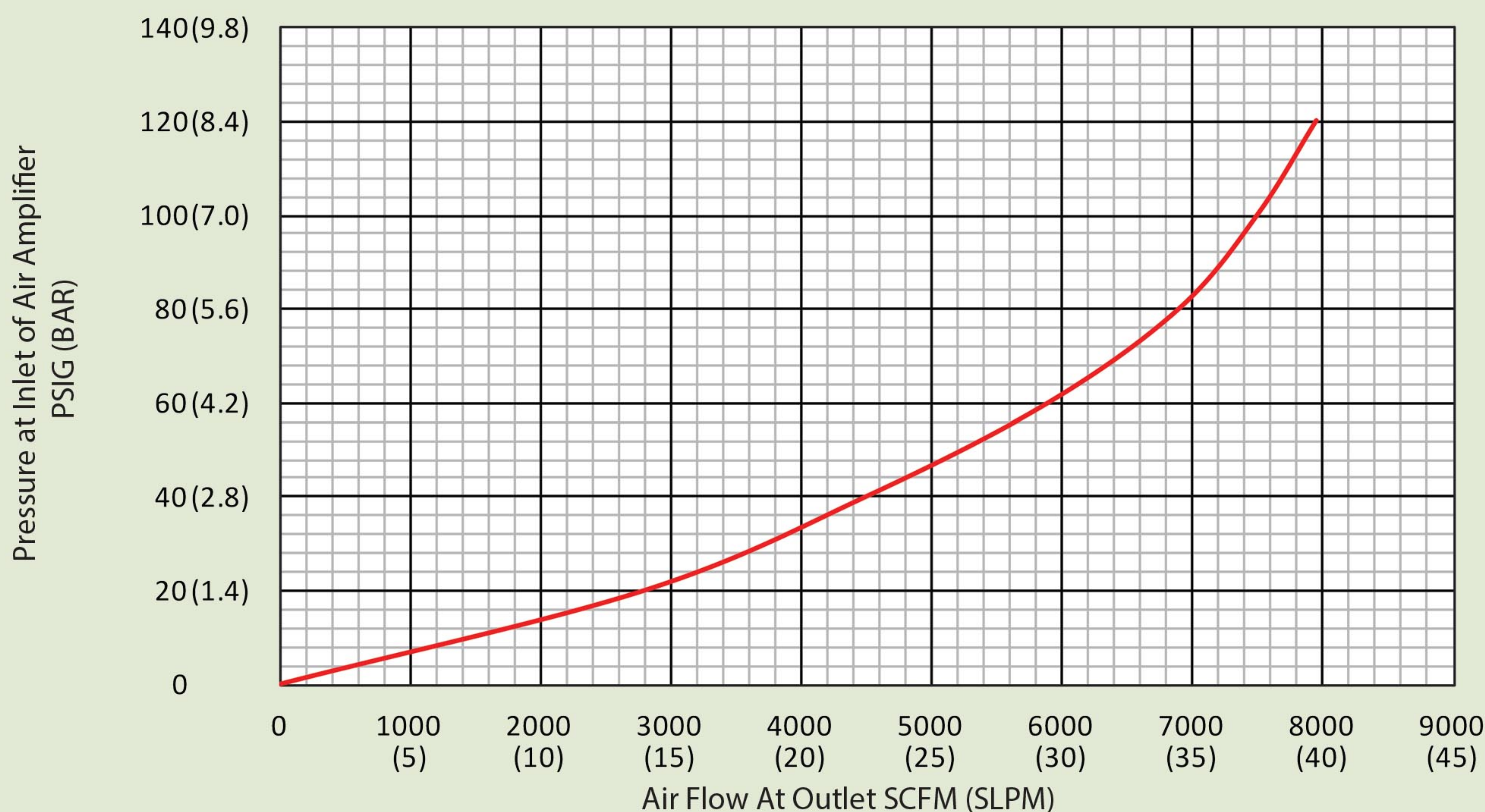
Pressure vs. Air Flow At Outlet for Model 40003 & 40003S Adjustable Air Amplifier
