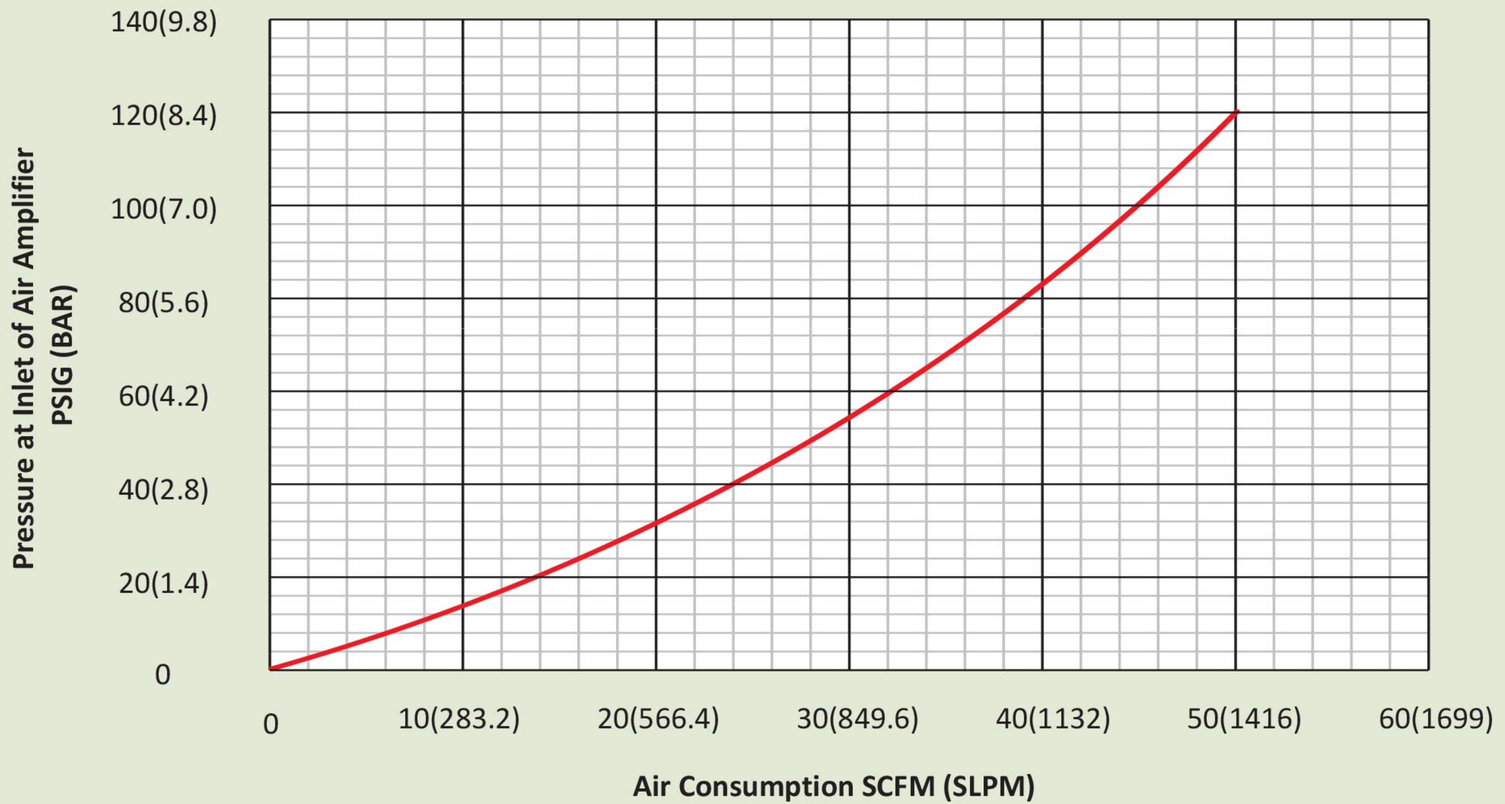
Pressure vs. Air Consumption for Model AM 75 Standard Air Amplifier
