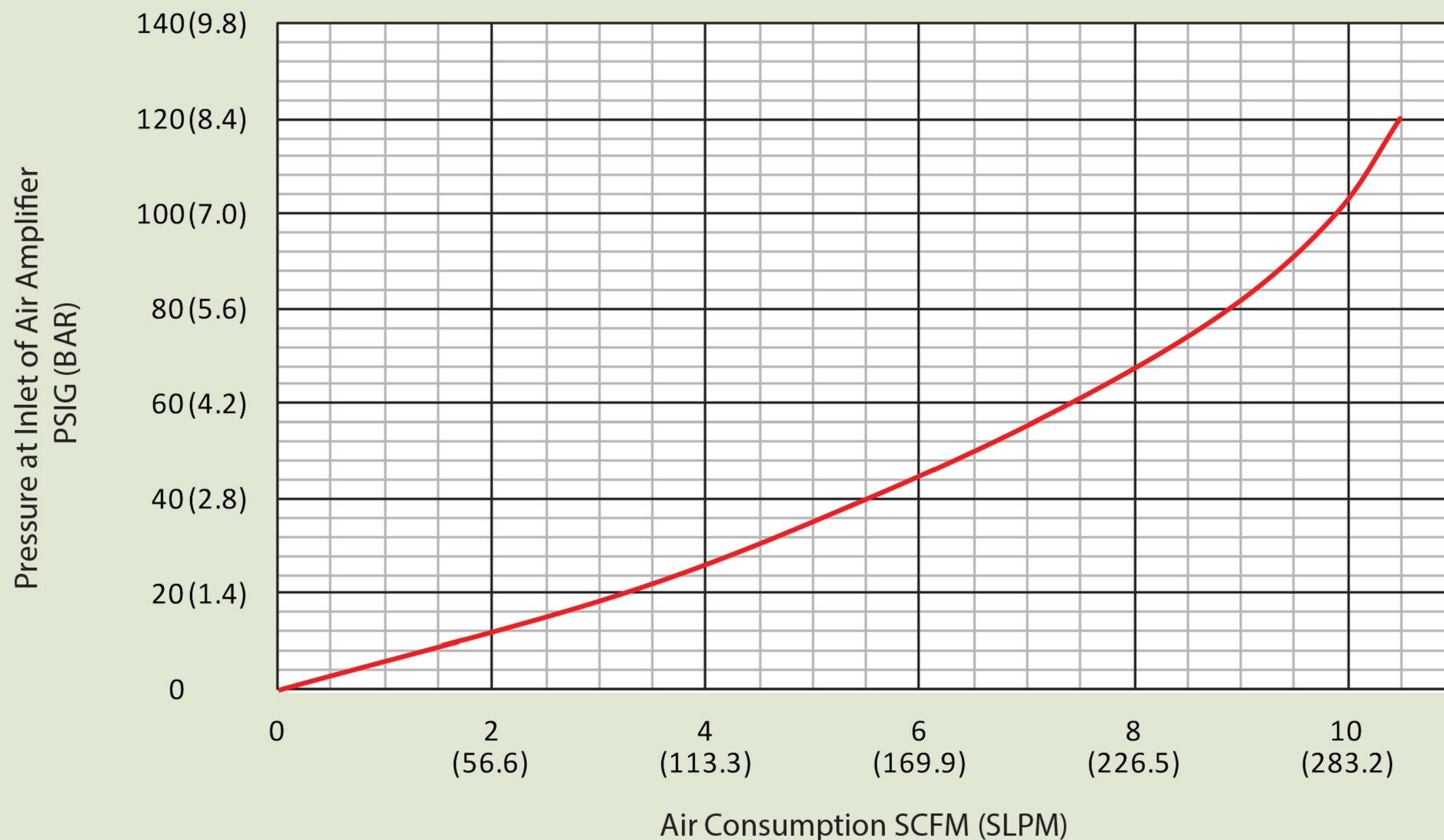
Pressure vs. Air Consumption for Model 40000 and 40000S Adjustable Air Amplifier
