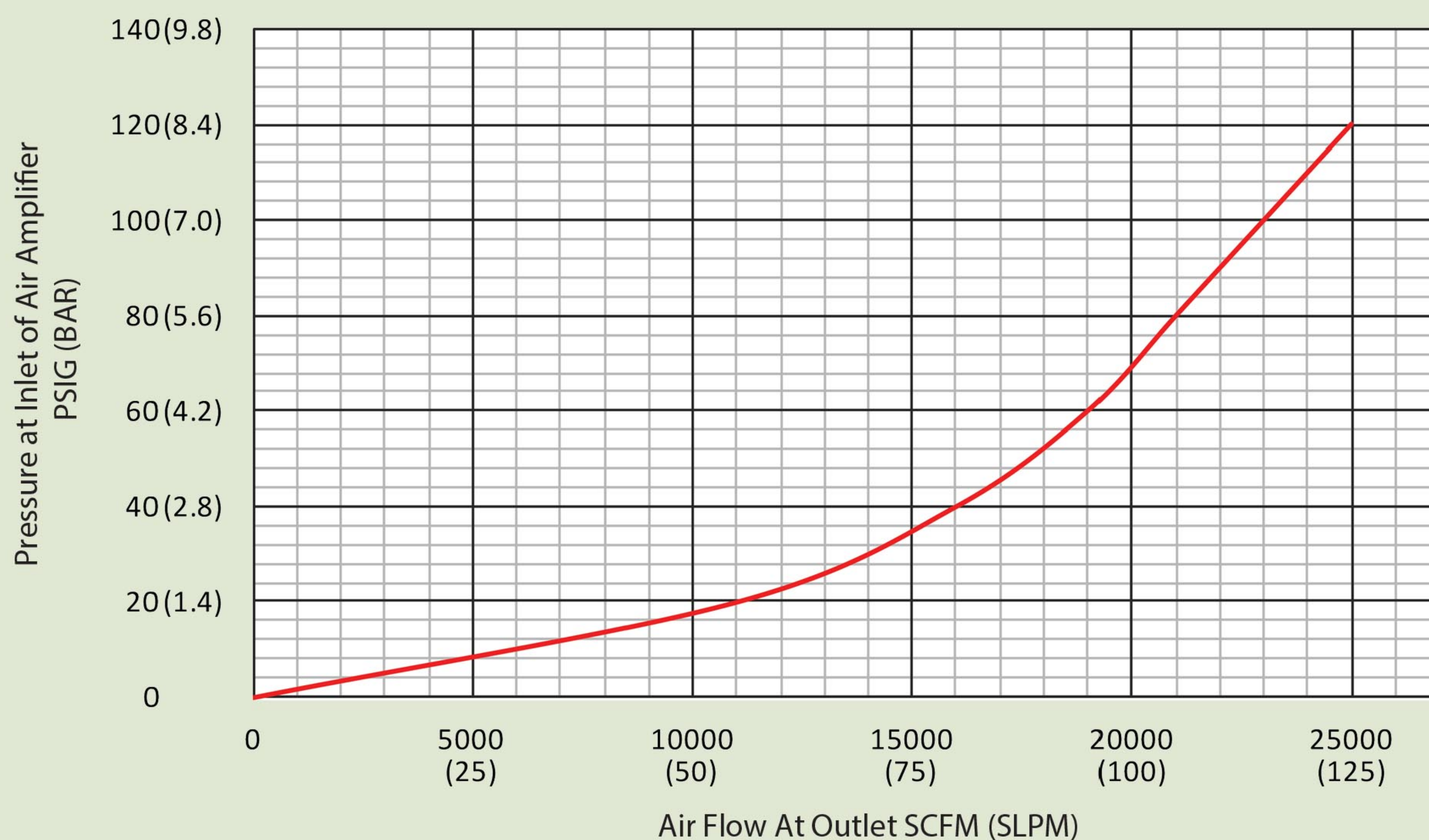
Pressure vs. Air Flow At Outlet for Model 40000 and 40000S Adjustable Air Amplifier
