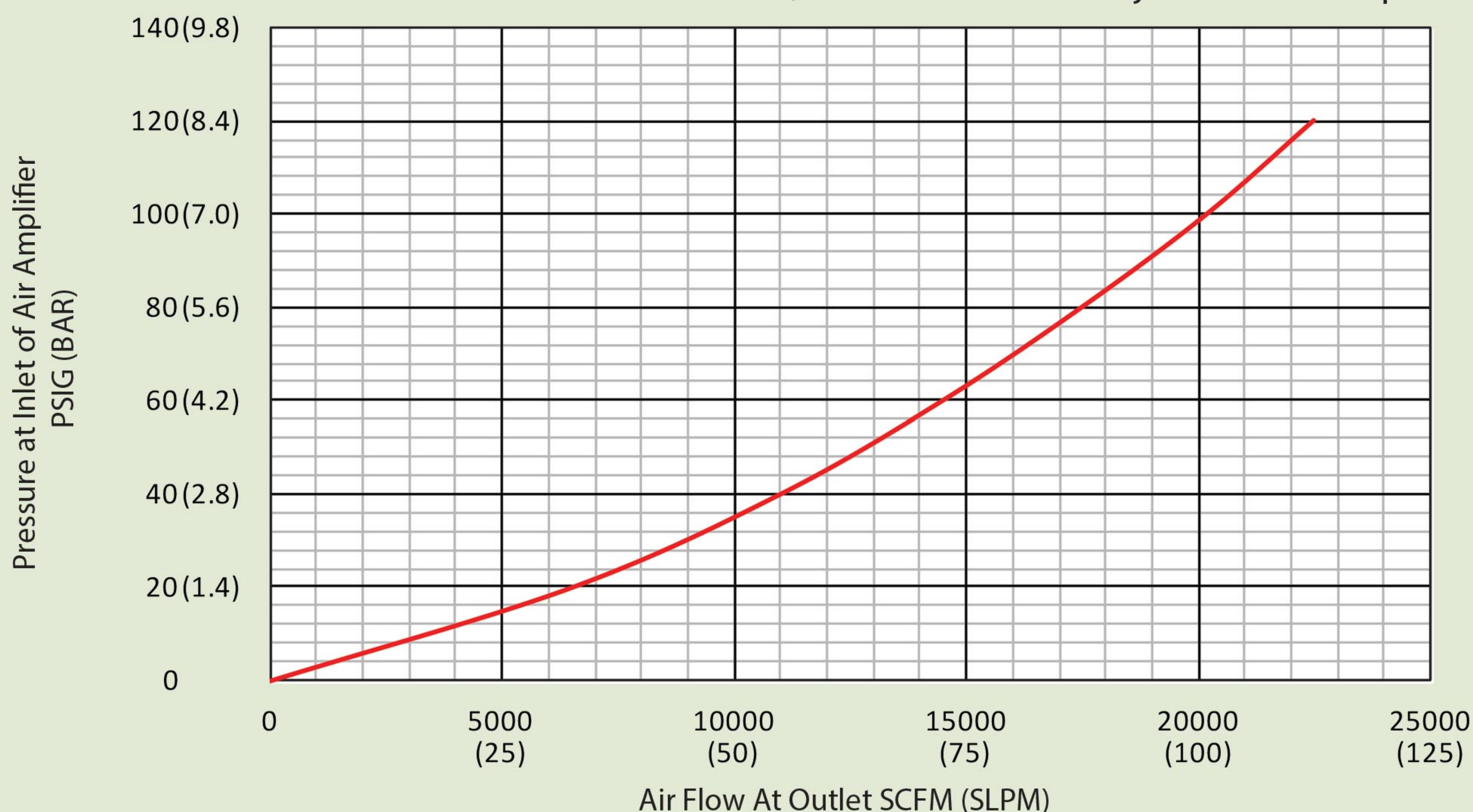
Pressure vs. Air Flow At Outlet for Model 40002, 40002G & 40002S Adjustable Air Amplifier
