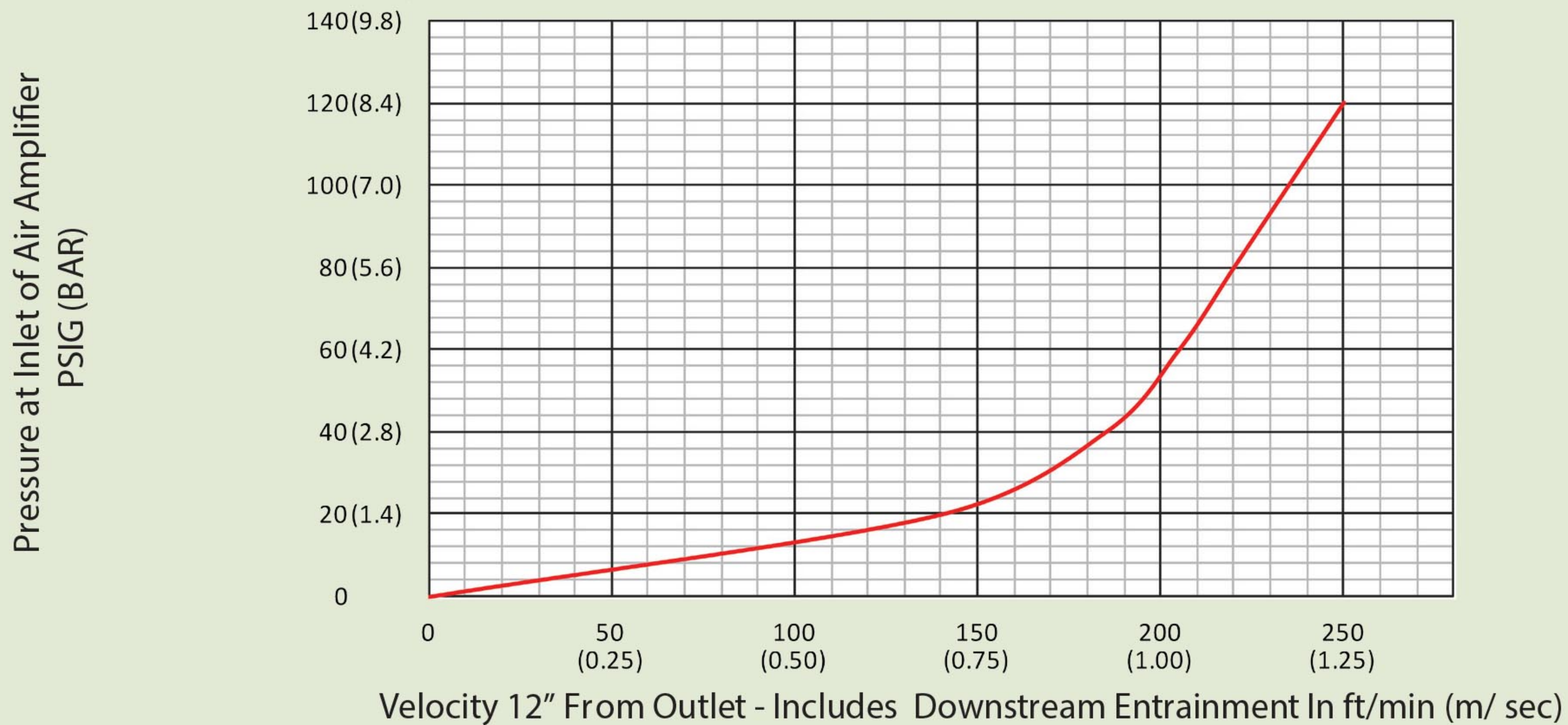
Pressure vs. Velocity 12" From Outlet for Model 40000 and 40000S Adjustable Air Amplifier
