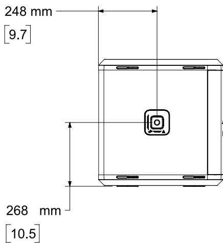
Left View
