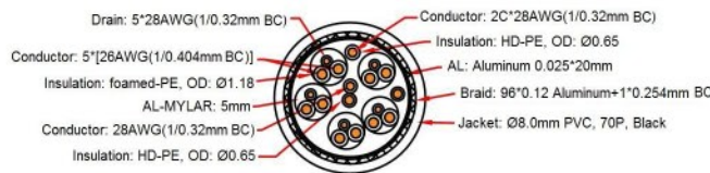
5P+4C(26AWG+28AWG)
