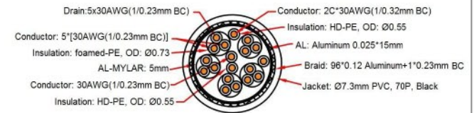
5P+4C(30AWG)
