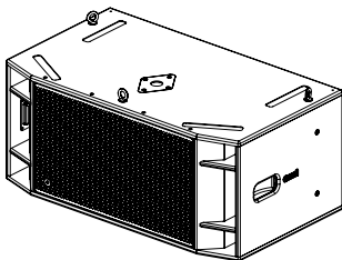
Drawing of HPI212S with eye bolt fly points
