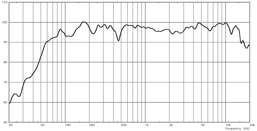
— HPI 110 - Frequency Response - 2.83V/1m
