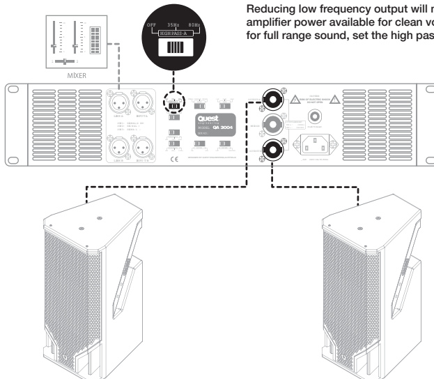
Recommended HPI110 Amplifier Configuration
