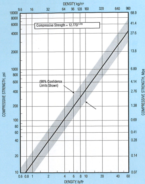
6.1 a Effect of density on compressive strength
