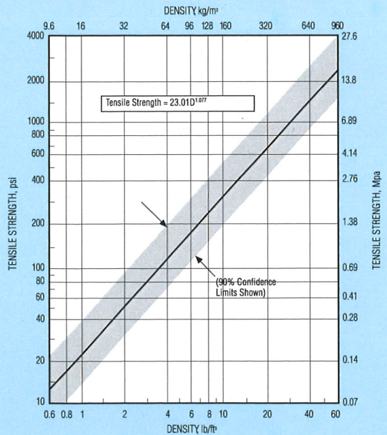
6.1 d Effect of density on tensile strength
