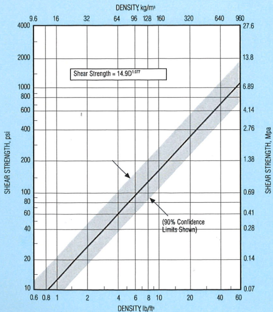
6.1 b Effect of density on shear strength
