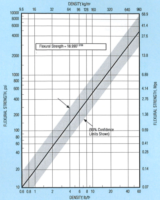
6.1 c Effect of density on flexural strength
