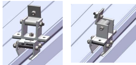
Figure 5 Front Leg Installation with Universal Klip-lok Interface
