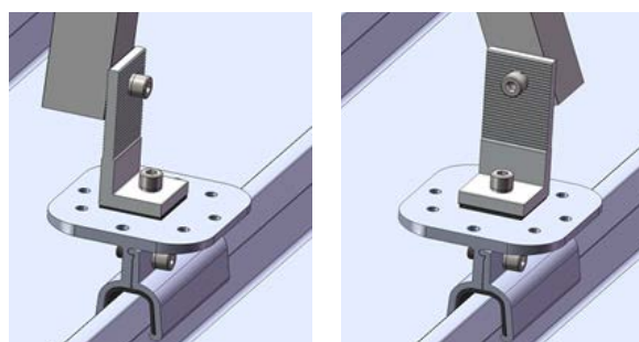
Figure 14 Tin Foot Rear Leg Installation with Other Klip-lok Interface
