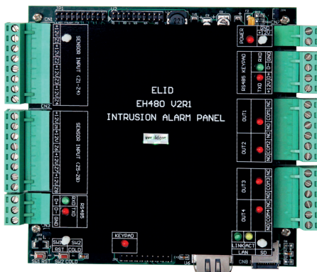
Controller Board
