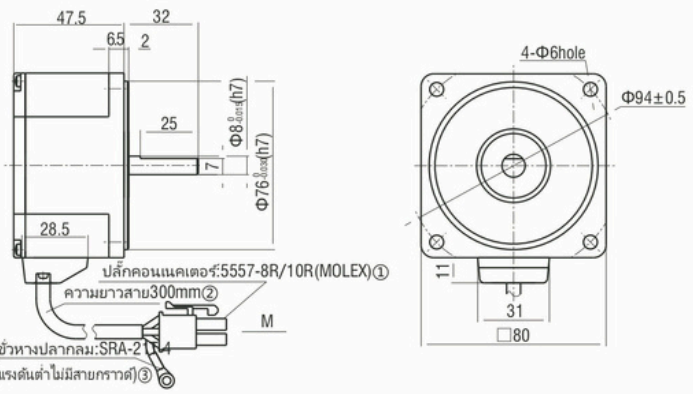
①Connector: 5557-8R/10R (MOLEX) ②The length of lead line 300mm ③Round terminal: SRA-21T-4 (No ground for low voltage)
