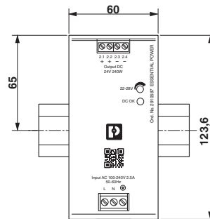
Dimensional drawing
