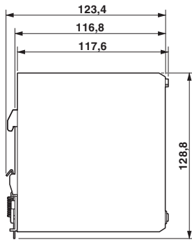
Dimensional drawing
