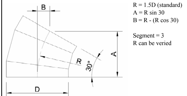
Curve Edge for U Clamp
