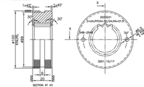
SHB-2548 J-3251 GO GAUGE
