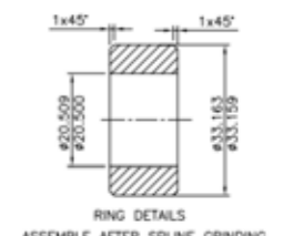
RING DETAILS ASSEMBLE AFTER SPLINE GRINDING
