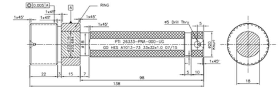
DRAWING FOR APPROVAL
